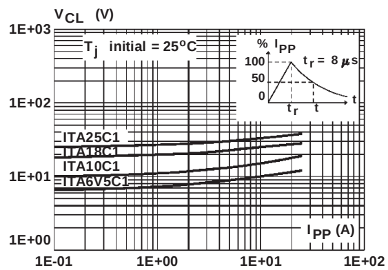
Fig.2 : Clamping voltage versus peak pulse current exponential waveform 8/20 \mu\text{s} .
